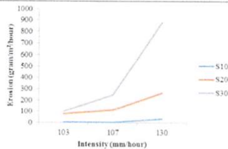
Figure 5. The effect of intensity on resulting erosion by using Vetiver bioengineering.
